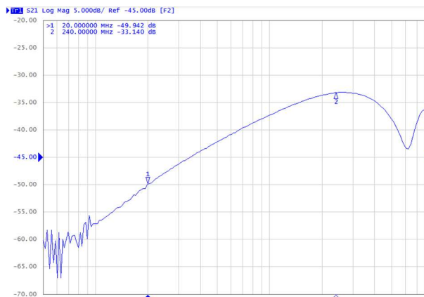
Off Isolation
