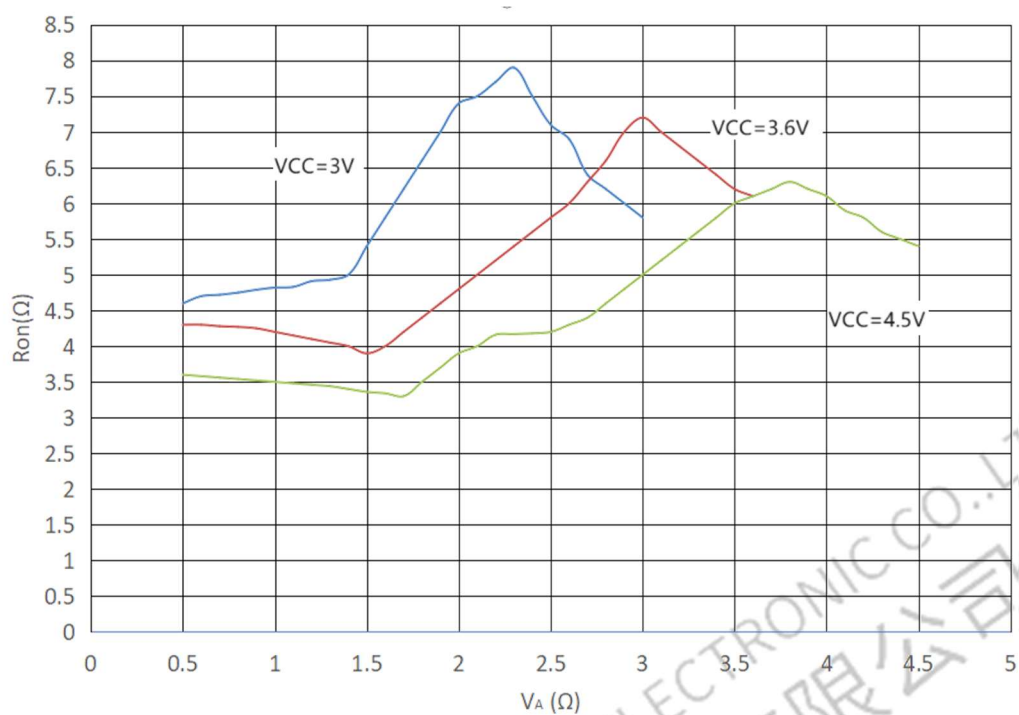
R_{on} vs. V_{CC} and V_A voltage
