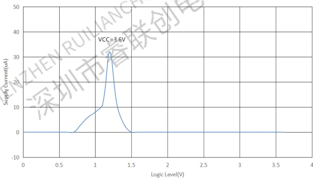
Supply Current vs. Logic Input
