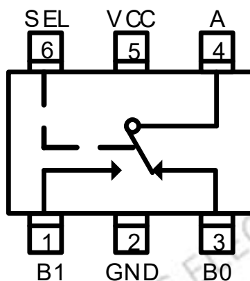
Pin configuration (Top view) SOT23-6
