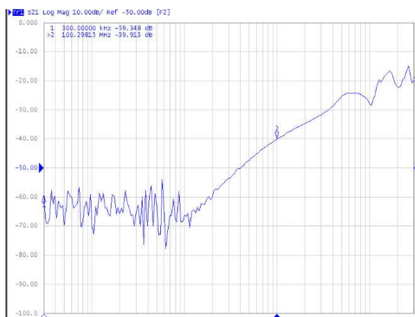
Cross-talk
